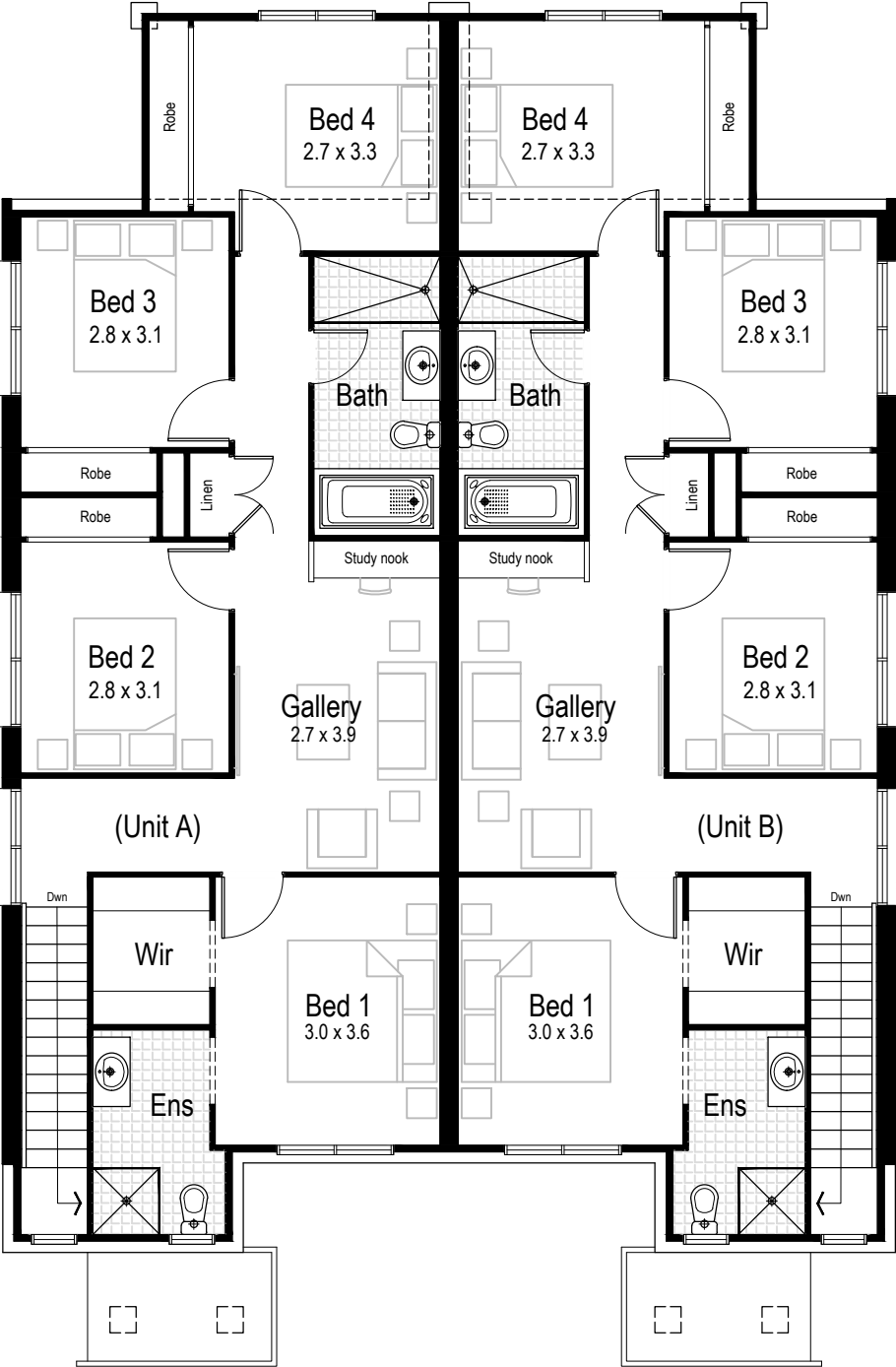
First Floor
